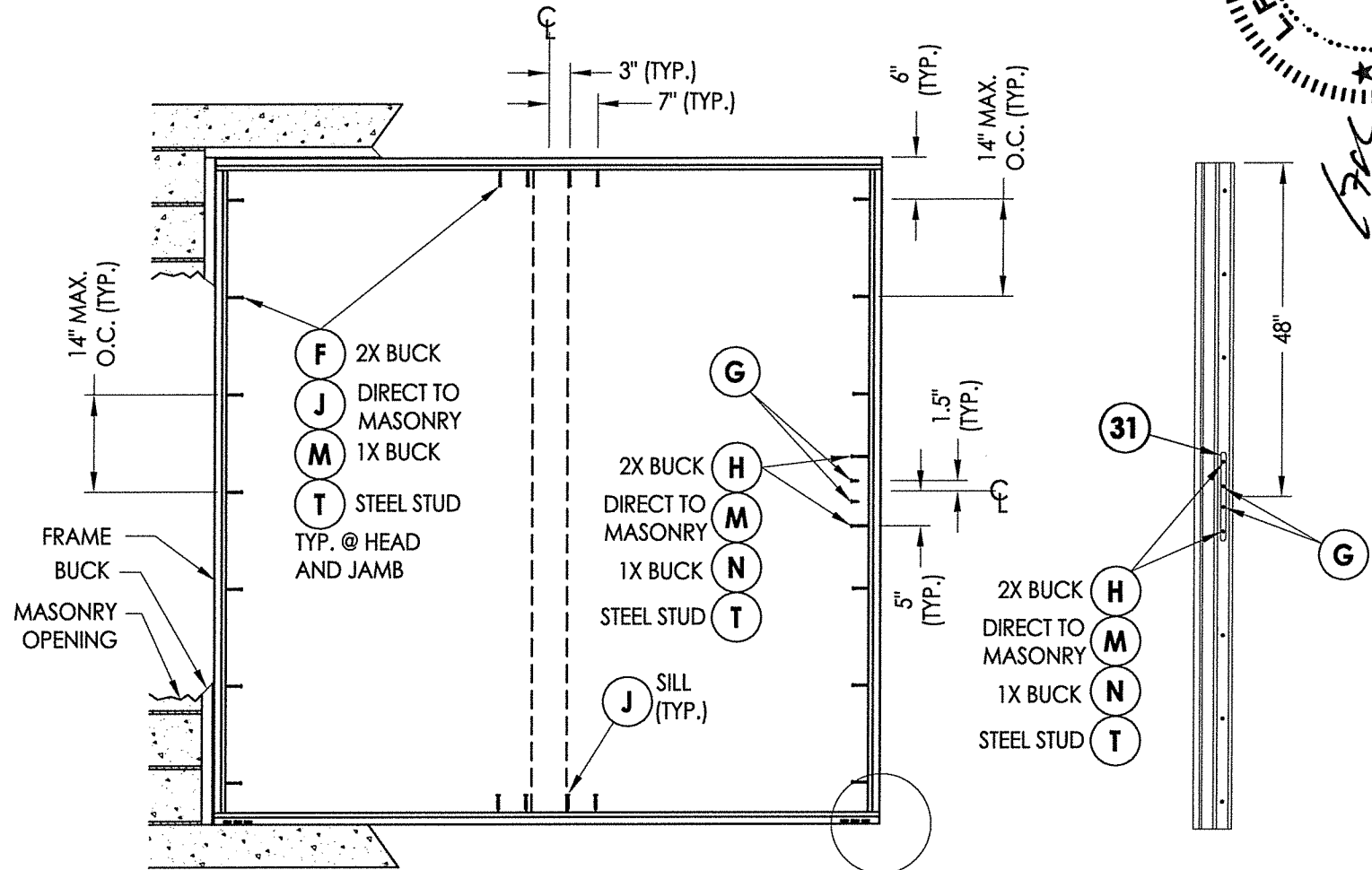
FRAME ANCHORING
